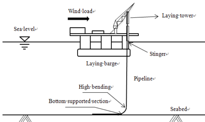
Figure 1. Diagram of the pipe laying by J type method.
